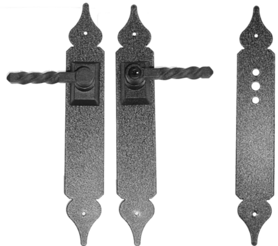
4" Twisted L Handle, blind mount, w/ 12 3/4" x 2" Escutcheon Plate 300-71168; Keyed Handle, 300-71150; Non-keyed Handle, 300-71155 Available as Double Auto Latch Kit 300-71170
